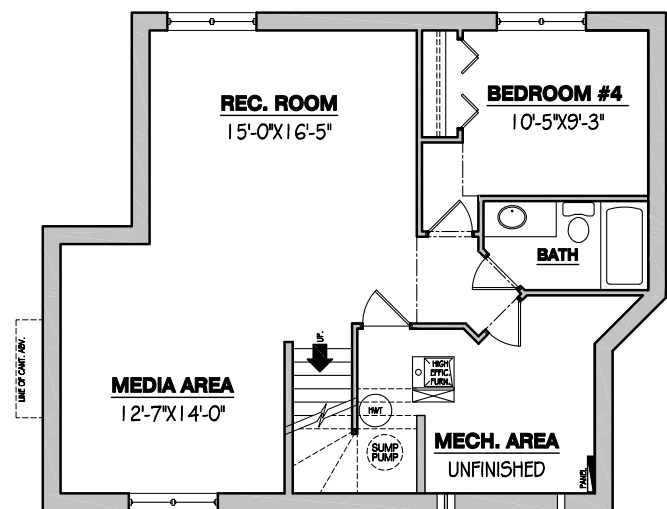
Future Basement Development 524 sq.ft.
