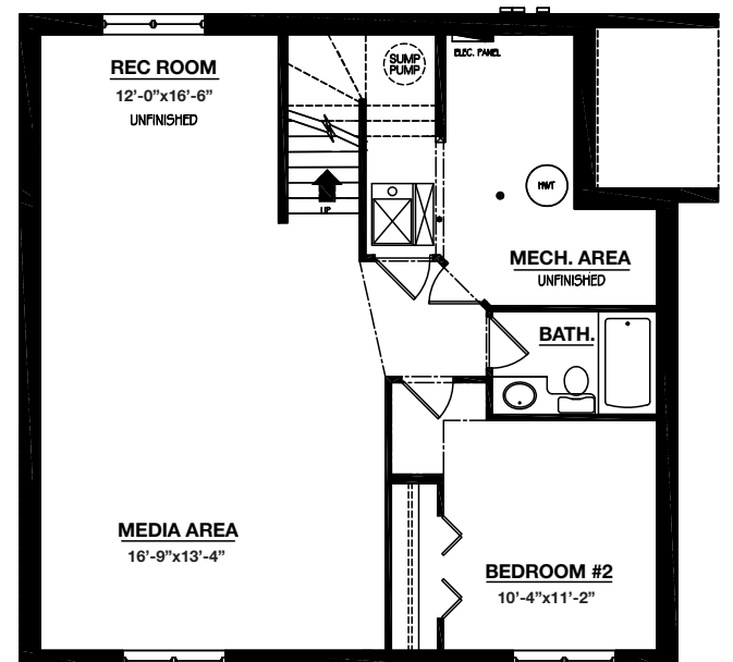
Future Basement Development 680 sq.ft.
